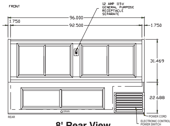
8' Rear View
